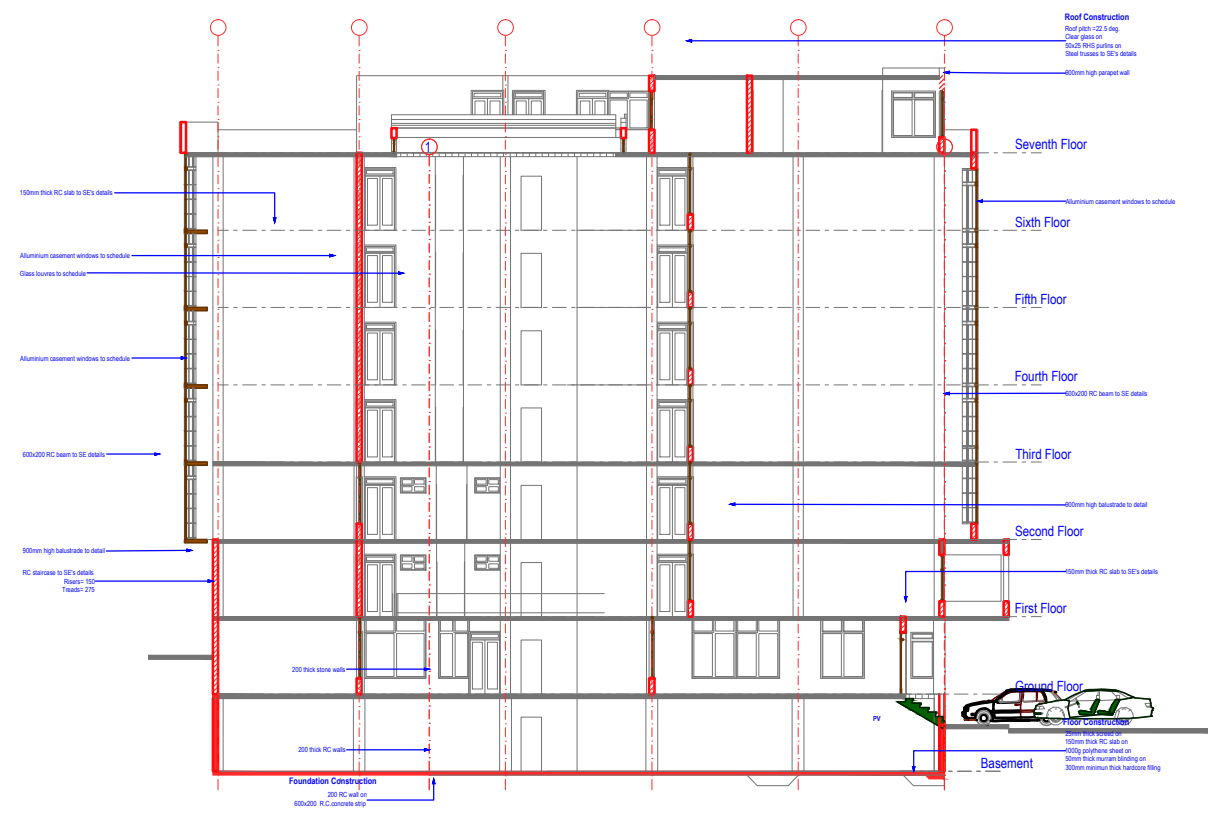
Section Y-Y
